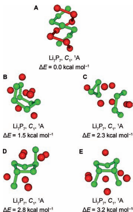
Figure 2. Representative optimized structures of \text{Li}_7\text{P}_7 , their point group symmetries, spectroscopic states, and ZPE-corrected (B3LYP/6-311 + G*) relative energies at the CCSD(T)/CBS//B3LYP/6-311 + G* level of theory (ZPE = zero-point corrected).
